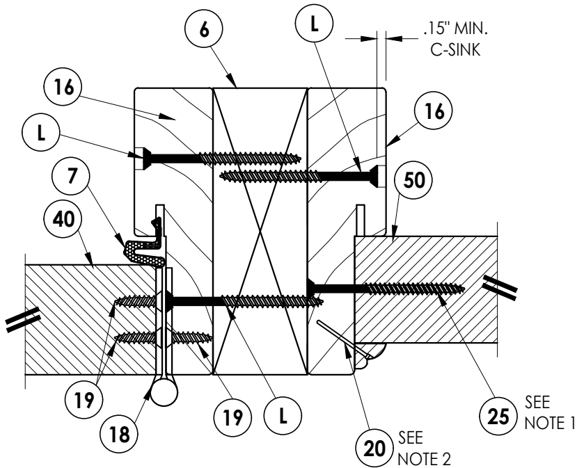
3 6 HORIZONTAL CROSS SECTION Inswing shown - outswing also approved
