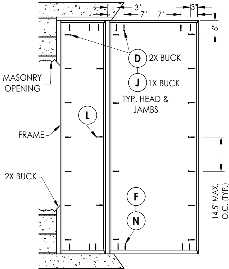
FRAME ANCHORING Masonry construction
