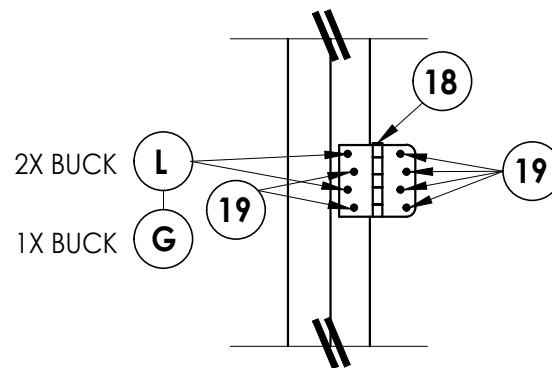
HINGE DETAIL
