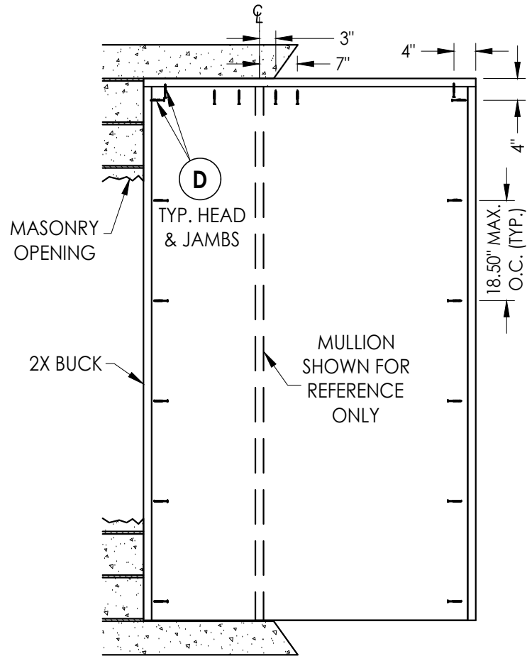
BUCK ANCHORING
