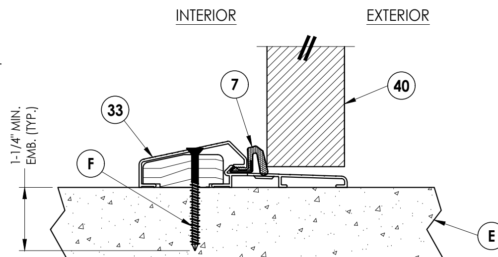
5 VERTICAL CROSS SECTION 7 Shown w/ ADA threshold
